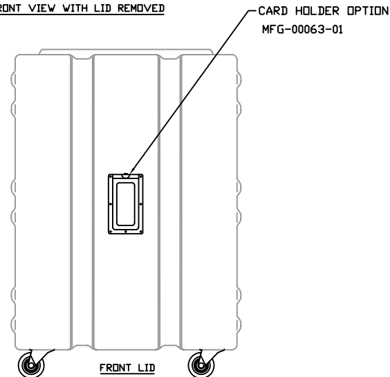
FRONT VIEW WITH LID REMOVED
