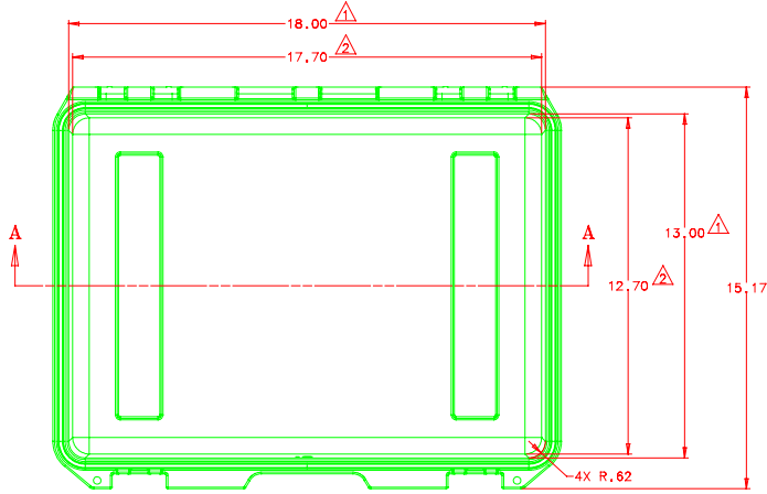
TOP VIEW SHOWN WITH LID REMOVED
